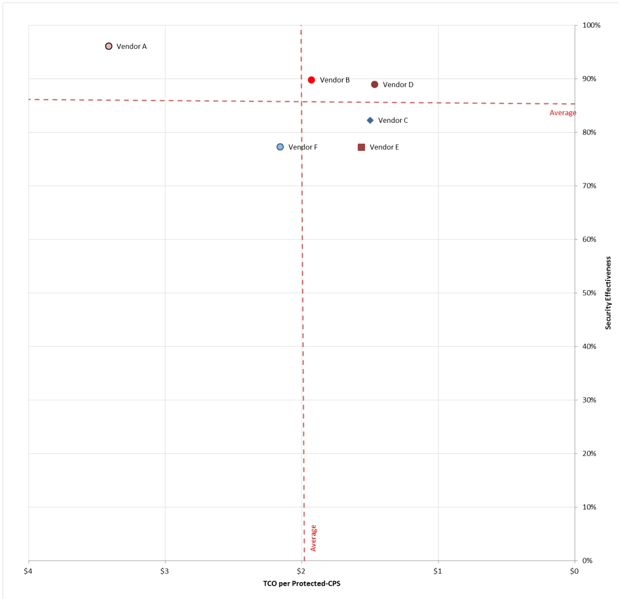
Figure 3 – Example SVM
